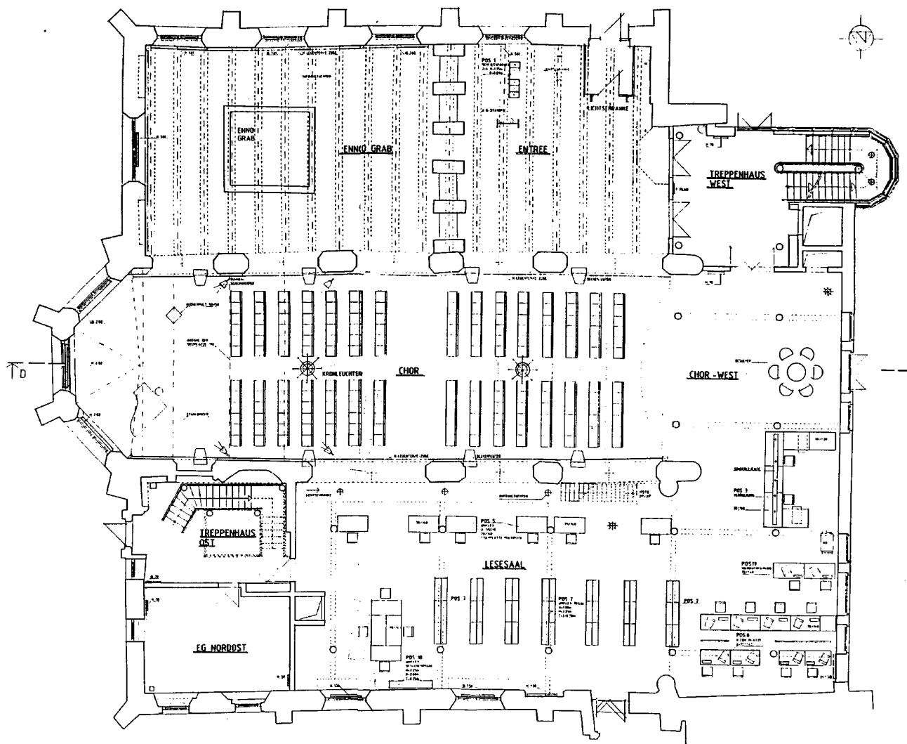
Grundriß Erdgeschoß
